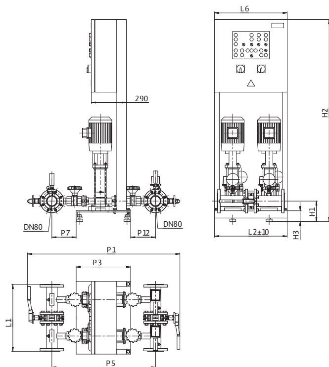
Wilo-CO 2 MVI 16...-6/SK-FFS-D-R
