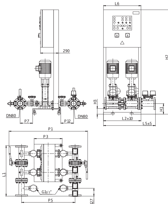
Wilo-CO 2 MVI 16...-6/SK-FFS-S-R
