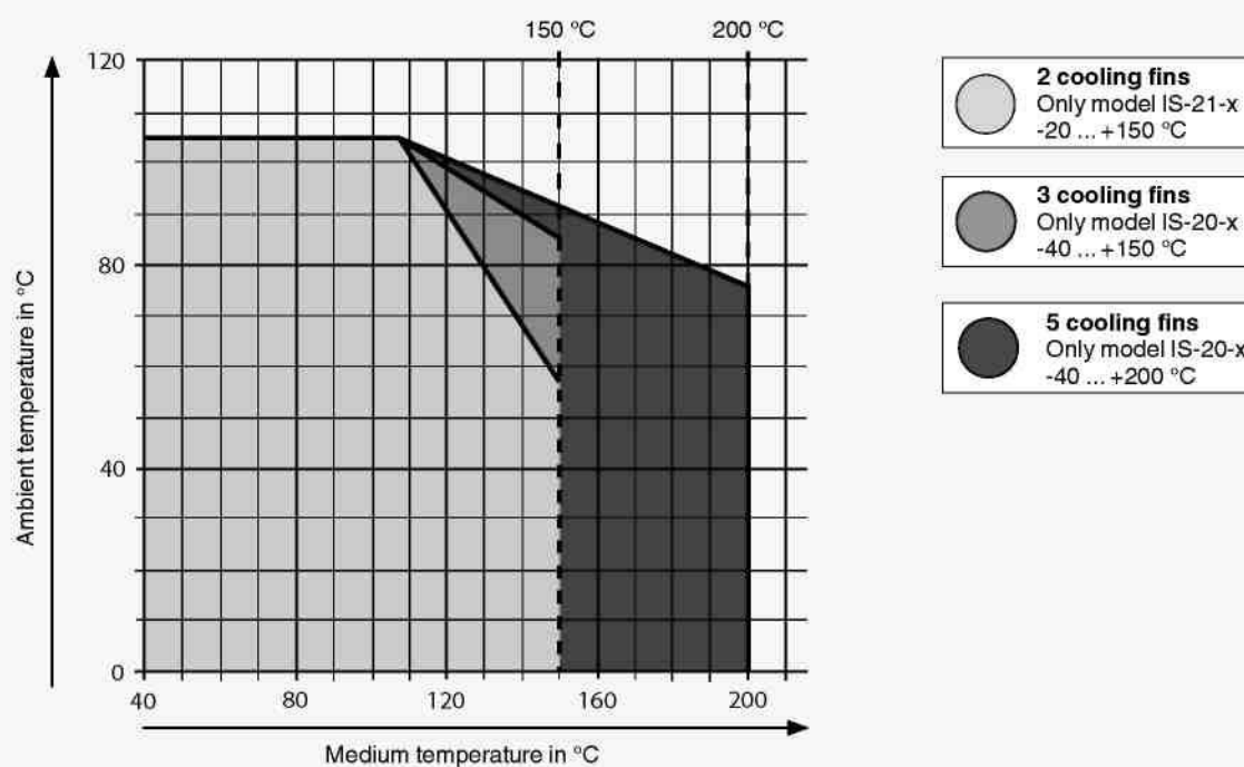
Permissible temperature ranges for process connections with cooling element
