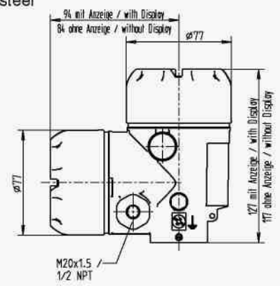
Dual chamber housing, cast stainless steel
