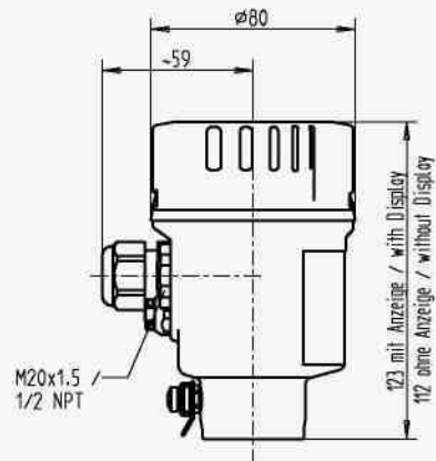
Single chamber housing, stainless steel, deep-drawn
